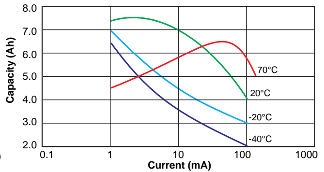
Capacity versus Current and Temperature
