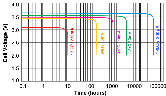
Typical discharge profile at 25°C
