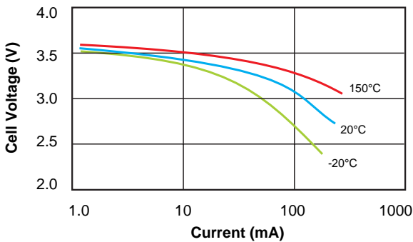
150°C Discharge Performance
