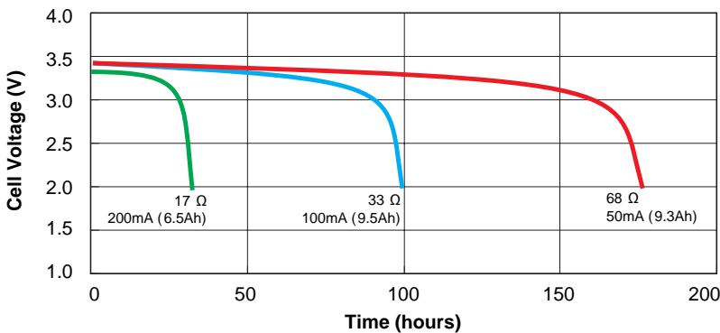
150°C Discharge Performance
