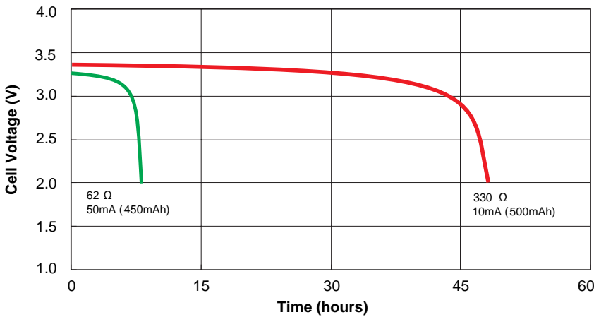
150°C Discharge Performance
